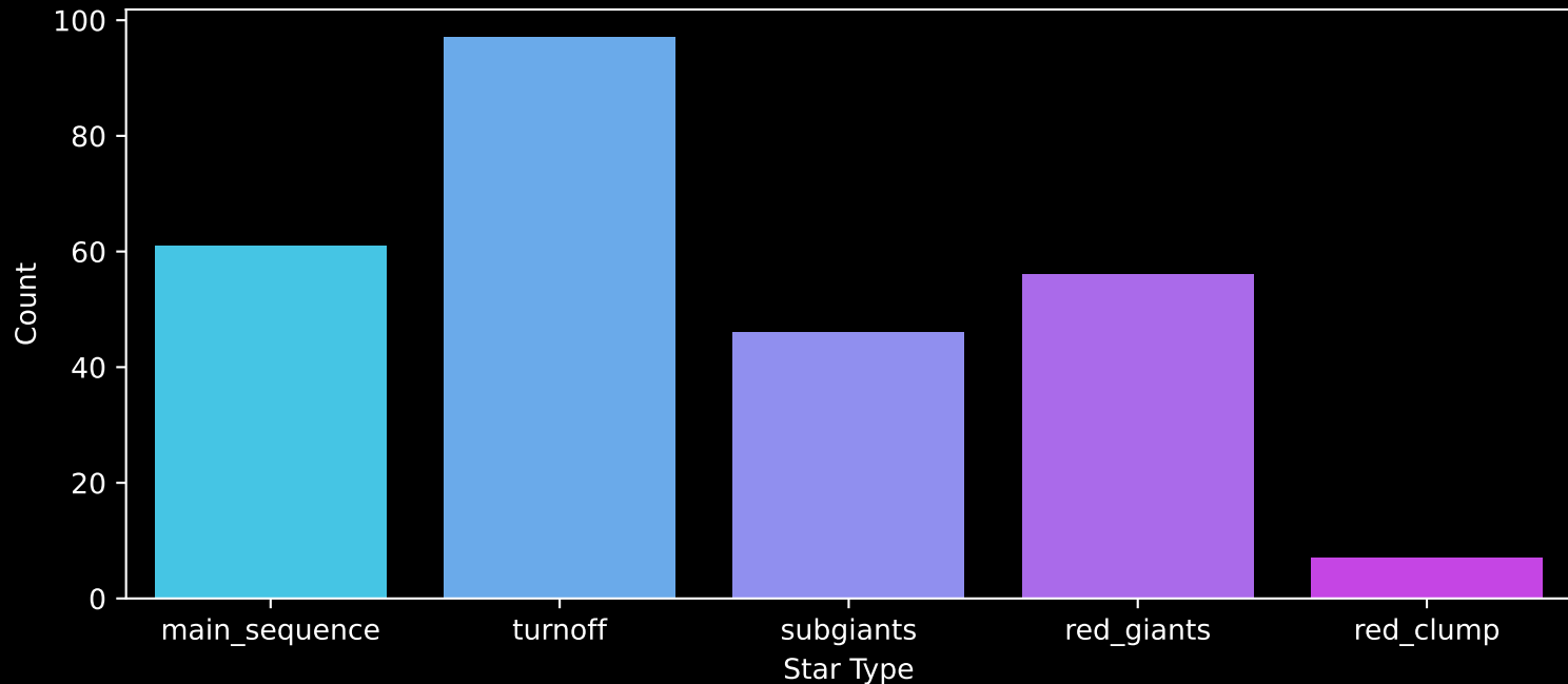
GALAH DR4 Field: [9276] Count plot of Star Type
