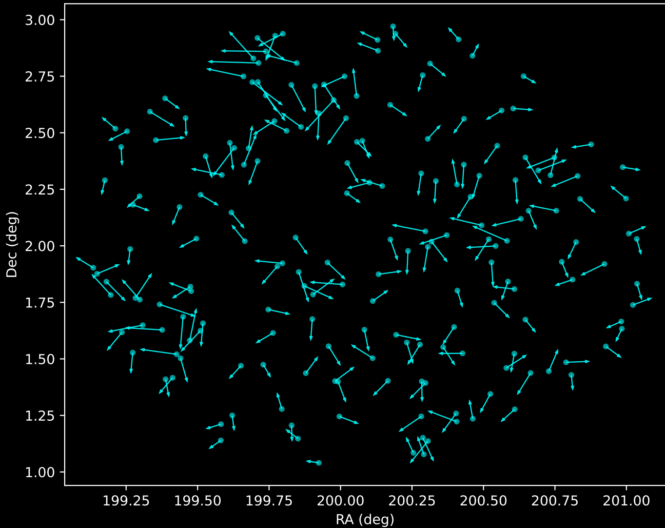
GALAH DR4 Noise Stream Proper Motion Vectors (n=187)
