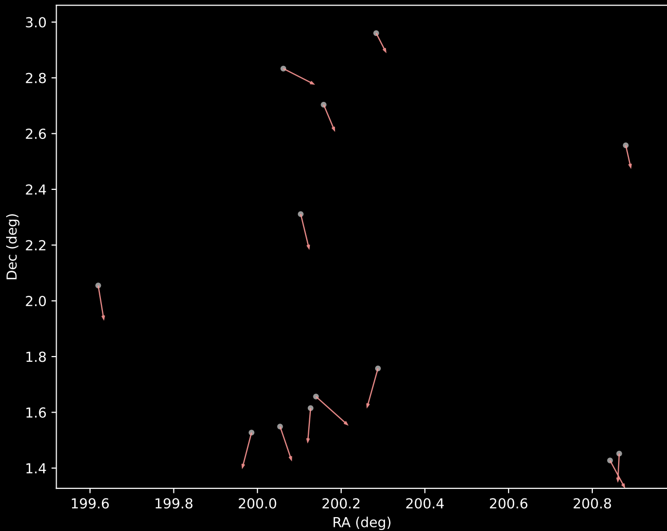
GALAH DR4 Cluster 7 Proper Motion Vectors (n=13)
