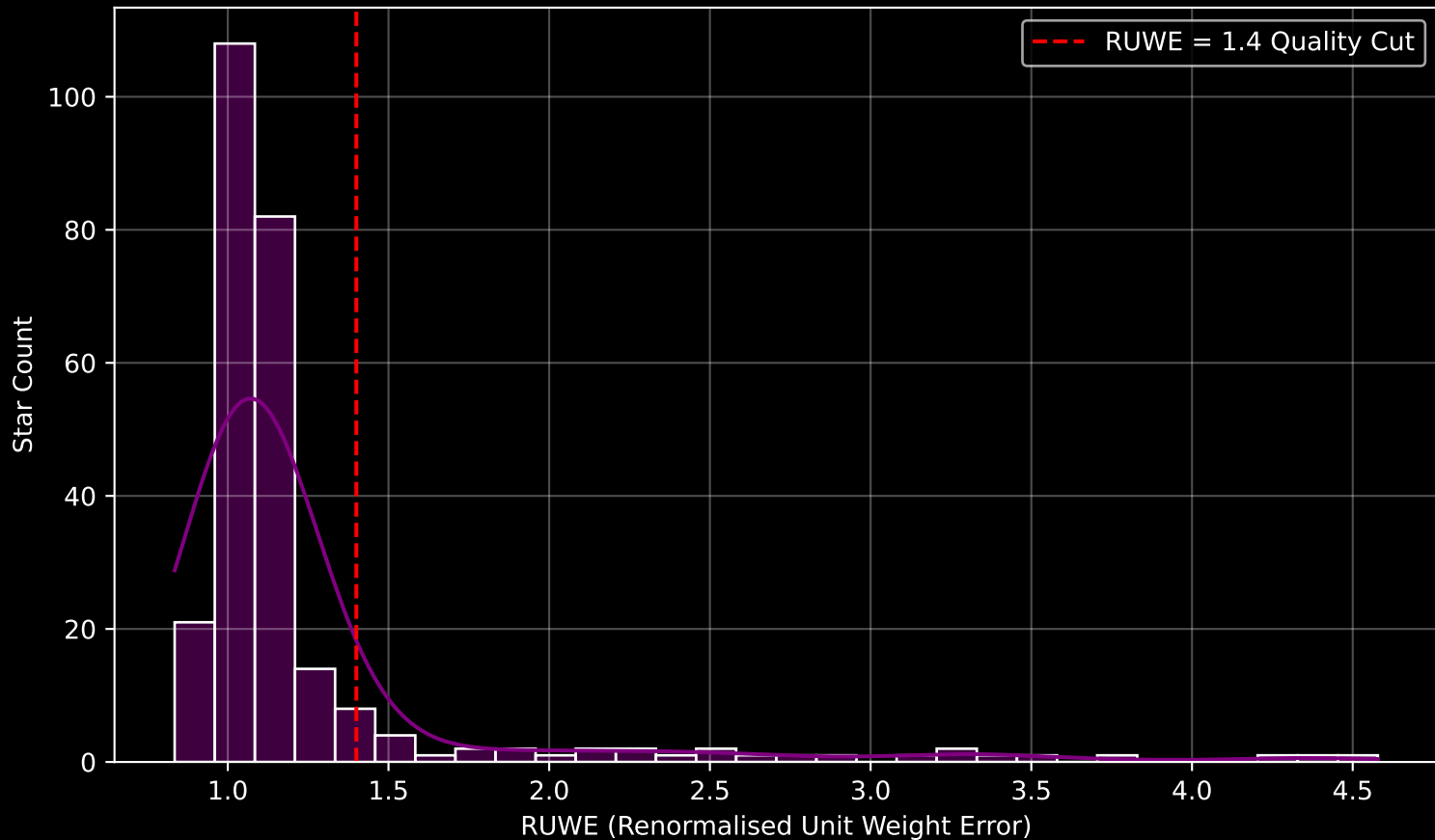
GALAH DR4 Field [9276] RUWE Distribution (n= 262)
