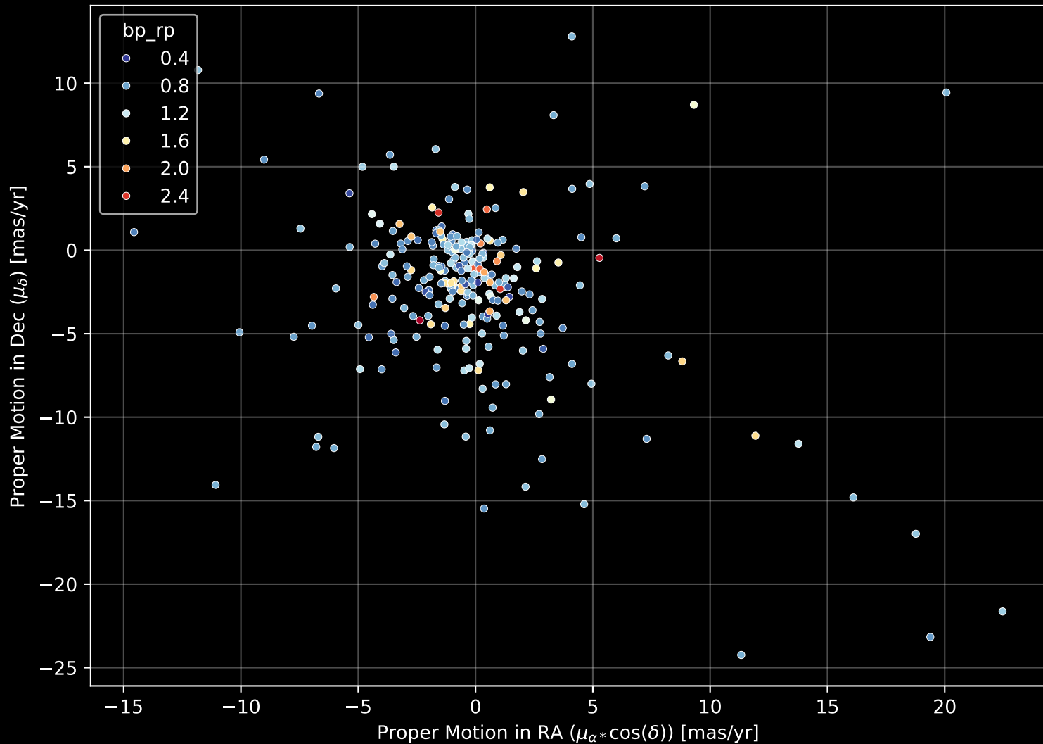
GALAH DR4 Field: [9276] Proper Motion Diagram (n= 267)
